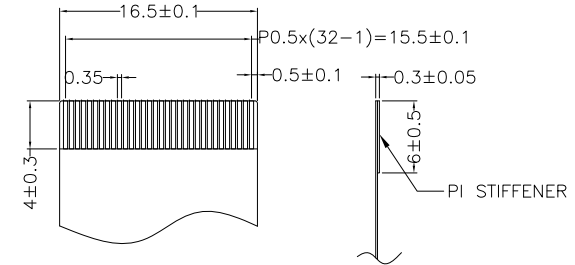
CN2 CONNECTOR MATED FPC/FFC STYLE (SCALE 2:1)
